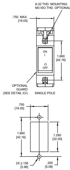
Panel Mounting Detail
